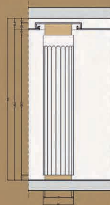
LIVING ROOM DECORATIVE COLUMN
